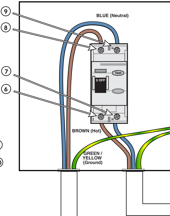
RCD Breaker Box
